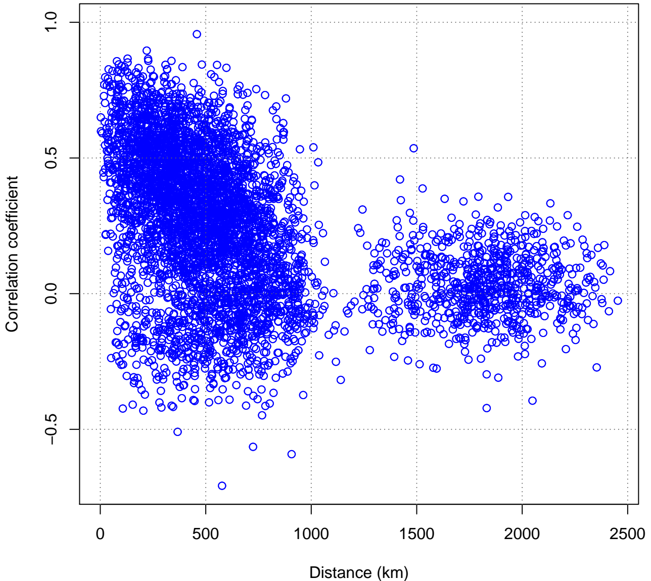
Correlogram of first difference 100 sampled series
