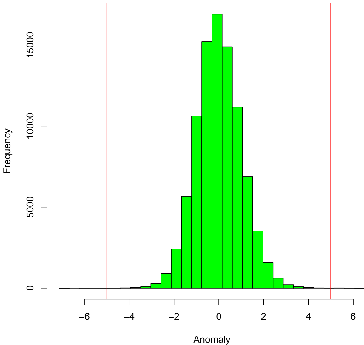
Histogram of normalized anomalies
