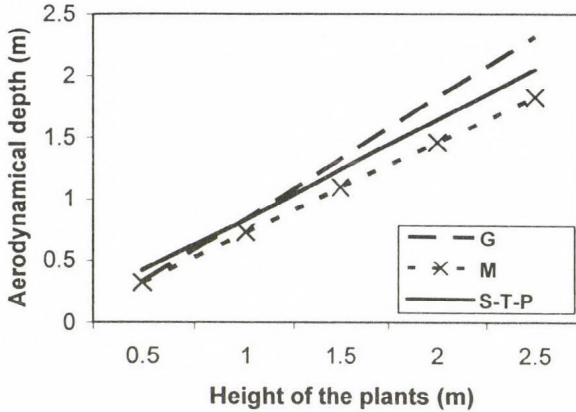
Fig. 2. Aerodynamical depth ( z_0 + d ) of the plant canopy versus plant height according to the different approaches G: Goudriaan (1977) , M: Monteith (1973) , S-T-P: Stanhill (1969) and Tanner and Pelton (1960) .
